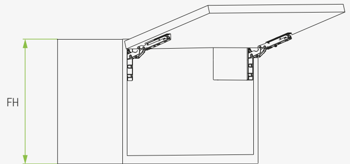
FH = Door Height
